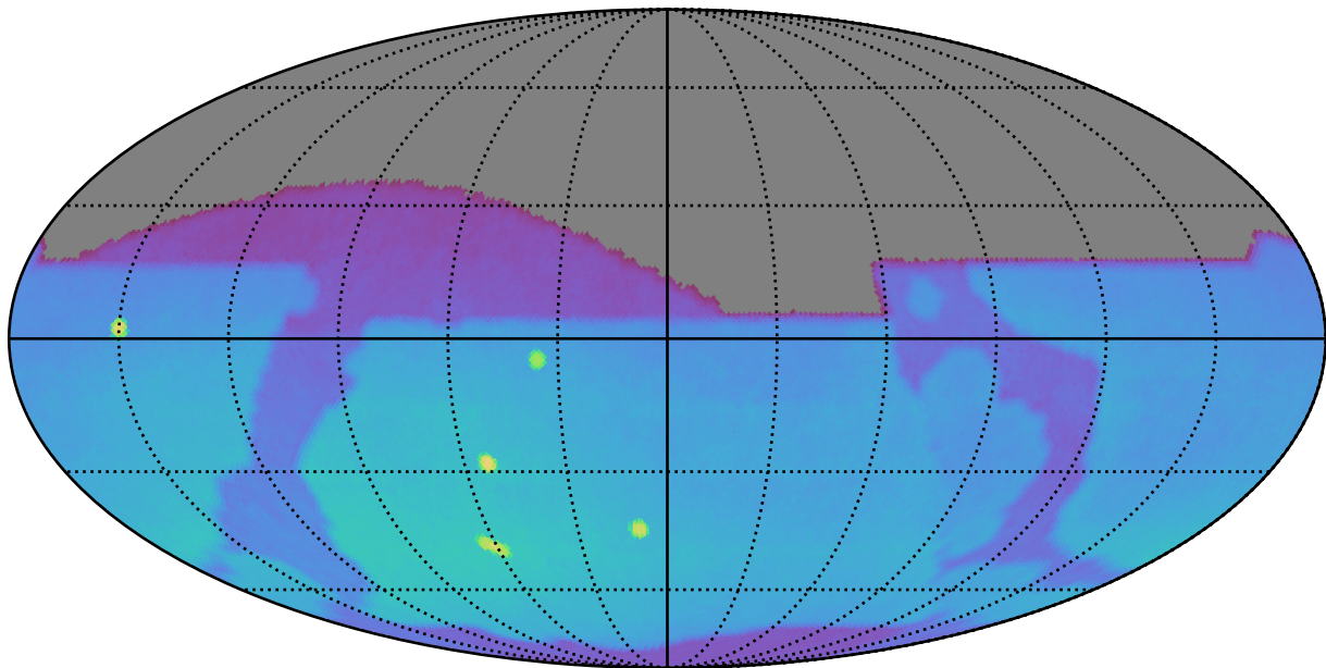
too_elab_r16_d2_ugrizy_v3.4_10yrs : Brown Dwarf, L4
