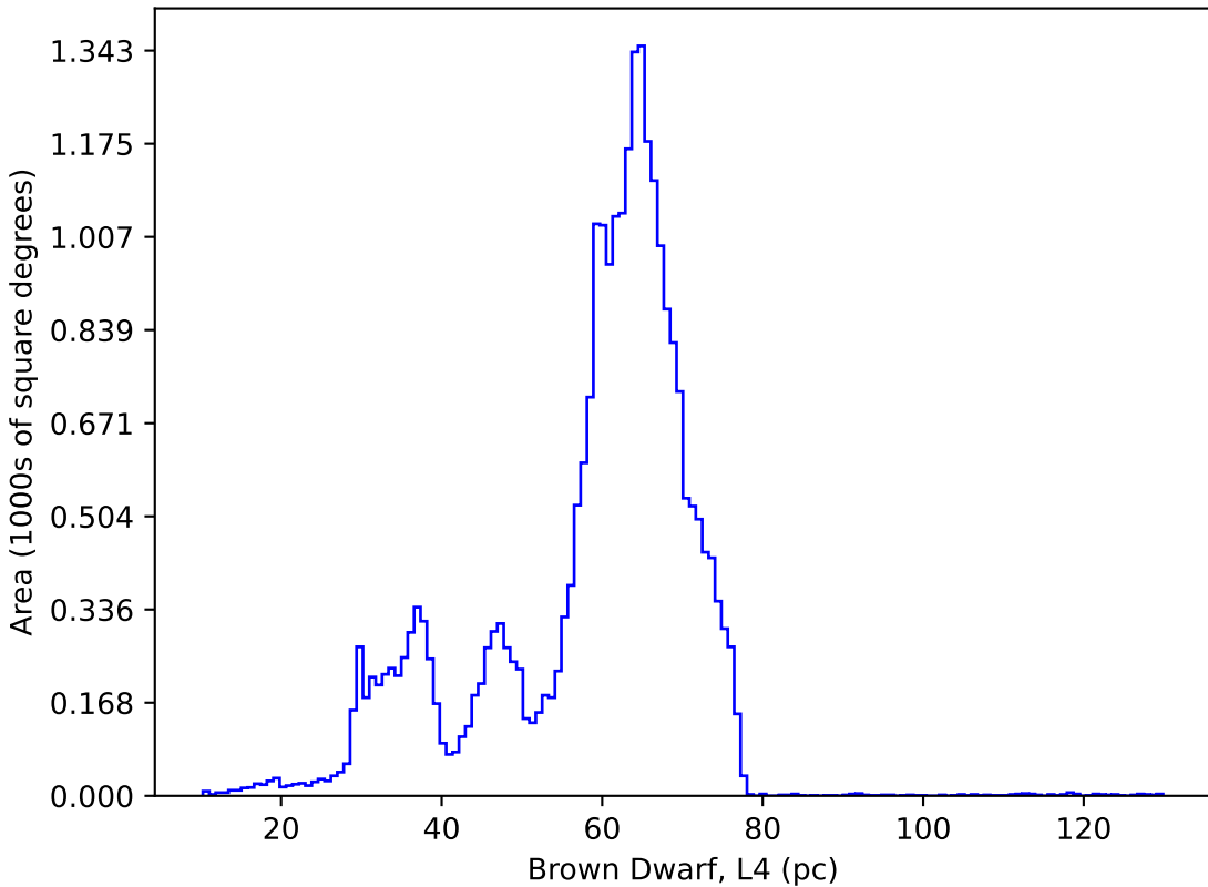
too_elab_r16_d2_ugrizy_v3.4_10yrs : Brown Dwarf, L4
