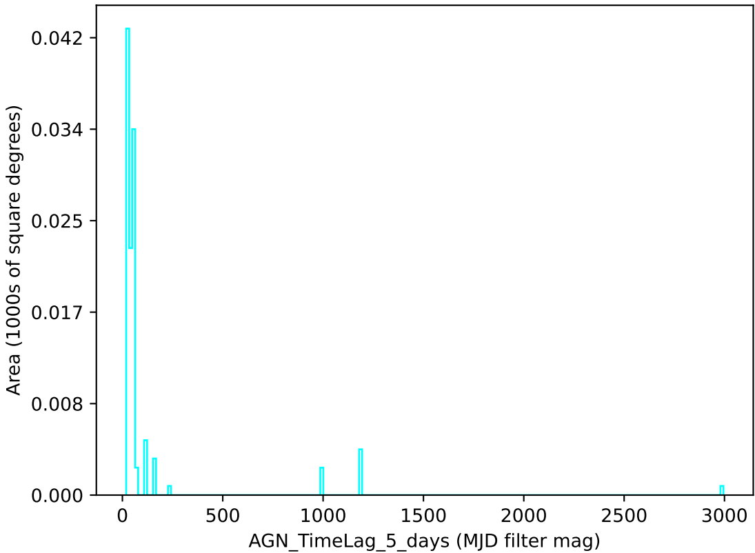
too_elab_r16_d2_ugrizy_v3.4_10yrs u band: AGN_TimeLag_5_days
