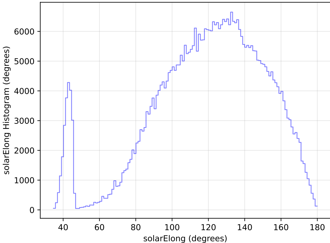
too_elab_r16_d2_ugrizy_v3.4_10yrs WFD z band: solarElong Histogram
