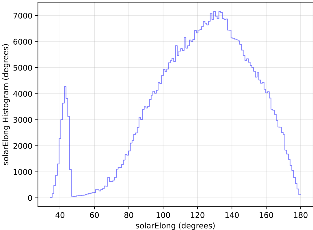
too_elab_r16_d2_ugrizy_v3.4_10yrs WFD i band: solarElong Histogram
