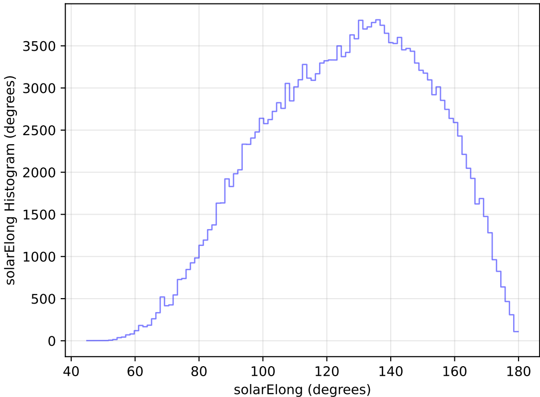
too_elab_r16_d2_ugrizy_v3.4_10yrs WFD g band: solarElong Histogram
