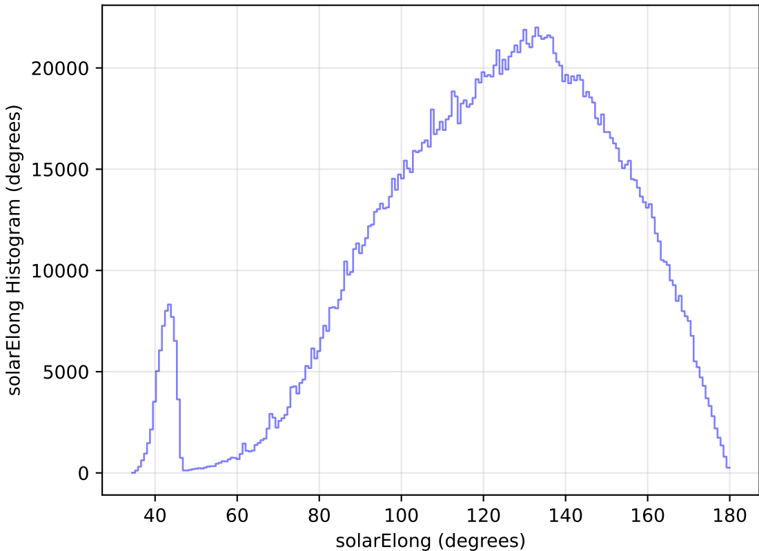
too_elab_r16_d2_ugrizy_v3.4_10yrs WFD all bands: solarElong Histogram
