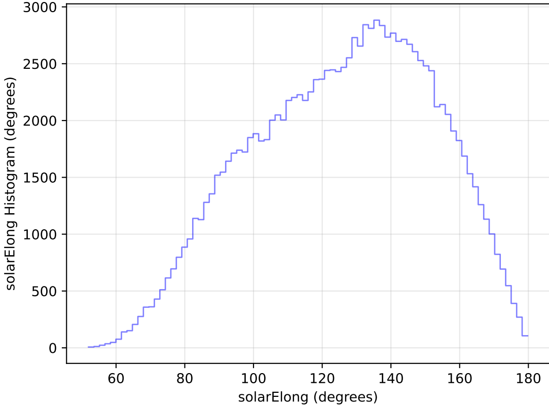
too_elab_r16_d2_ugrizy_v3.4_10yrs All sky u band: solarElong Histogram
