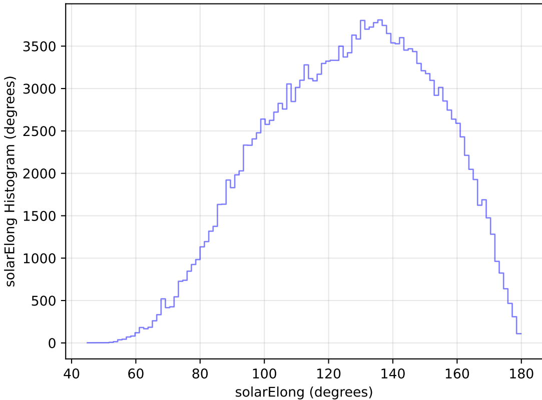
too_elab_r16_d2_ugrizy_v3.4_10yrs All sky g band: solarElong Histogram
