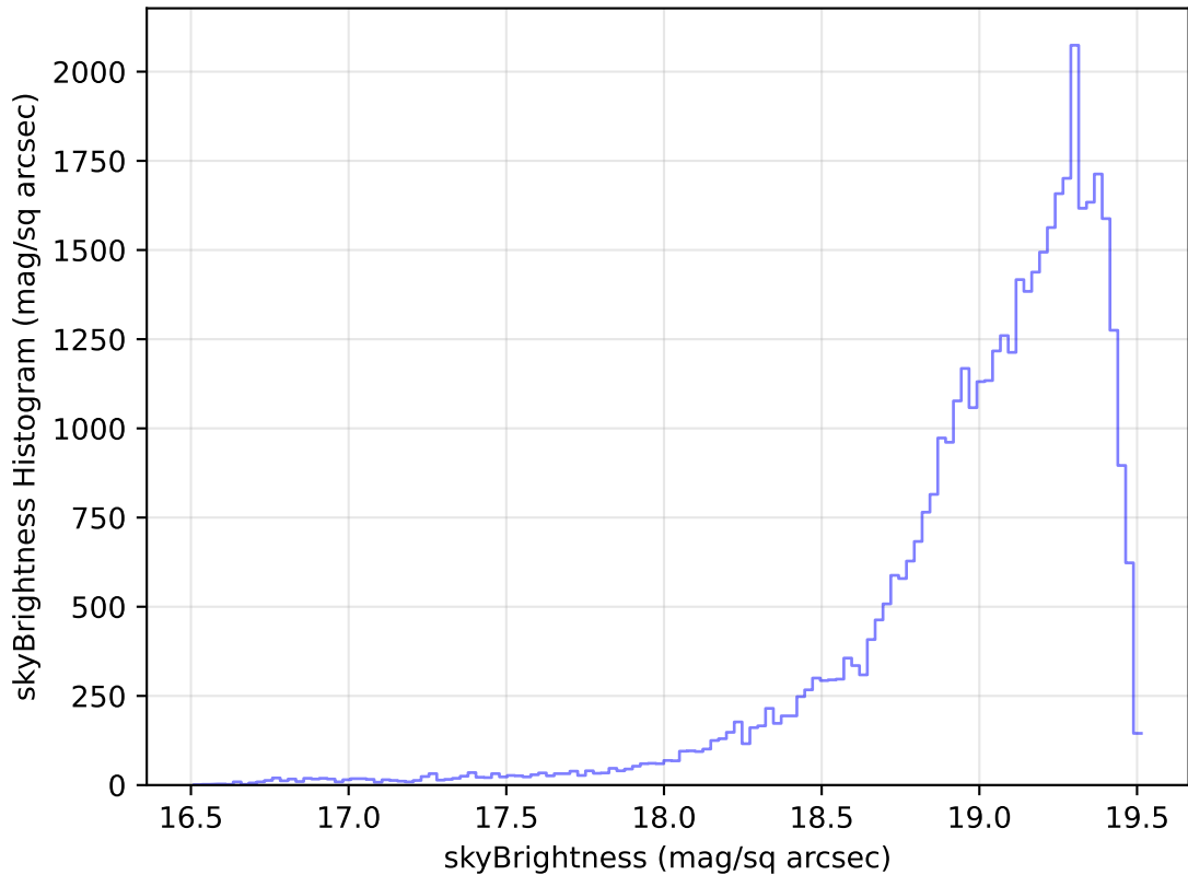
too_elab_r16_d2_ugrizy_v3.4_10yrs Yr 1 z band: skyBrightness Histogram
