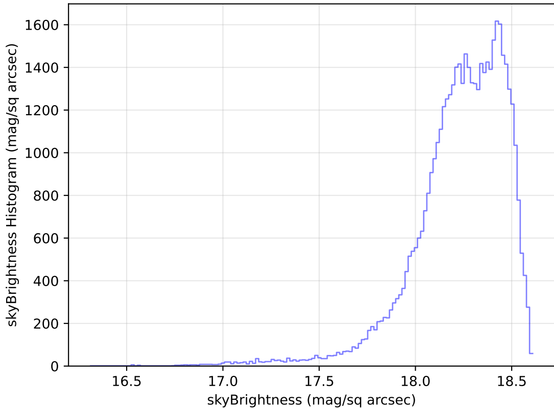
too_elab_r16_d2_ugrizy_v3.4_10yrs Yr 1 y band: skyBrightness Histogram
