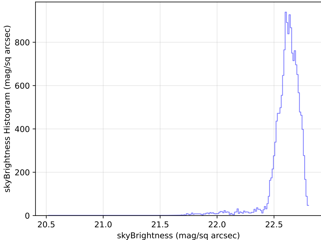
too_elab_r16_d2_ugrizy_v3.4_10yrs Yr 1 u band: skyBrightness Histogram
