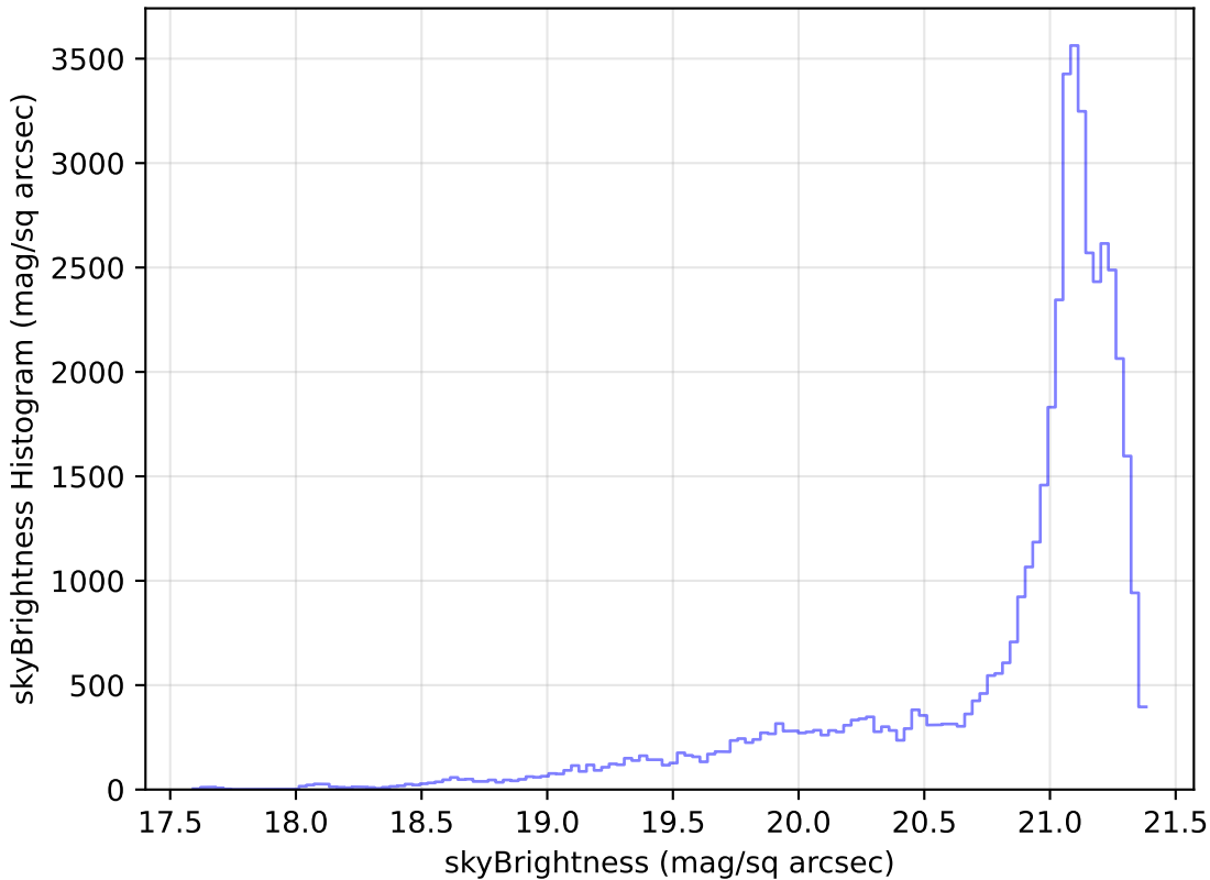
too_elab_r16_d2_ugrizy_v3.4_10yrs Yr 1 r band: skyBrightness Histogram
