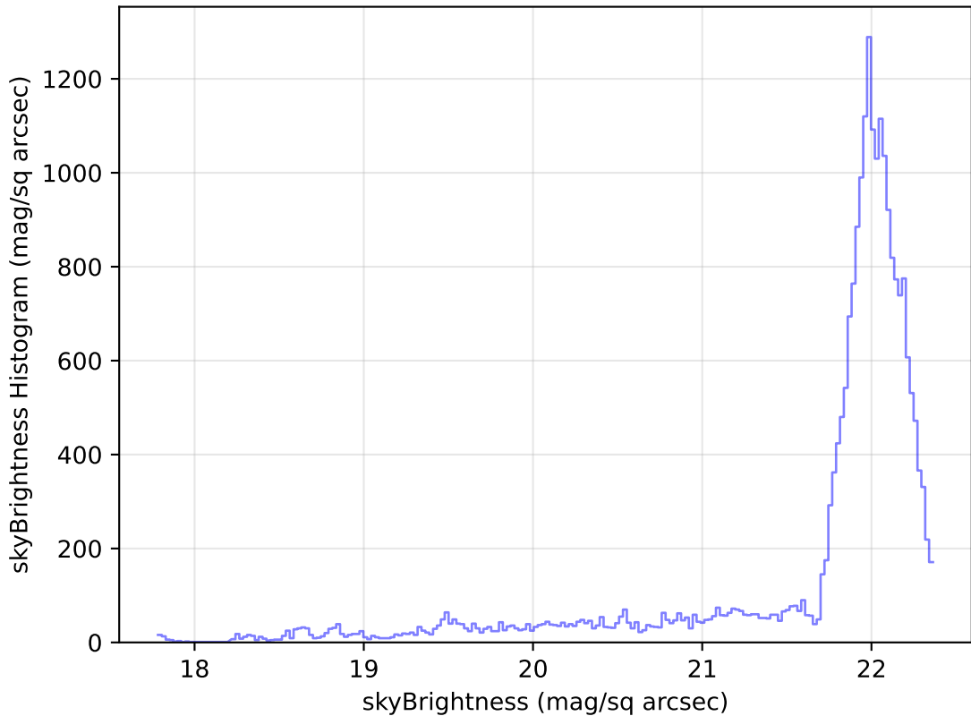
too_elab_r16_d2_ugrizy_v3.4_10yrs Yr 1 g band: skyBrightness Histogram
