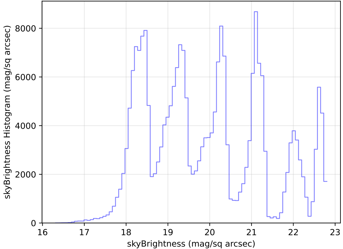
too_elab_r16_d2_ugrizy_v3.4_10yrs Yr 1 all bands: skyBrightness Histogram
