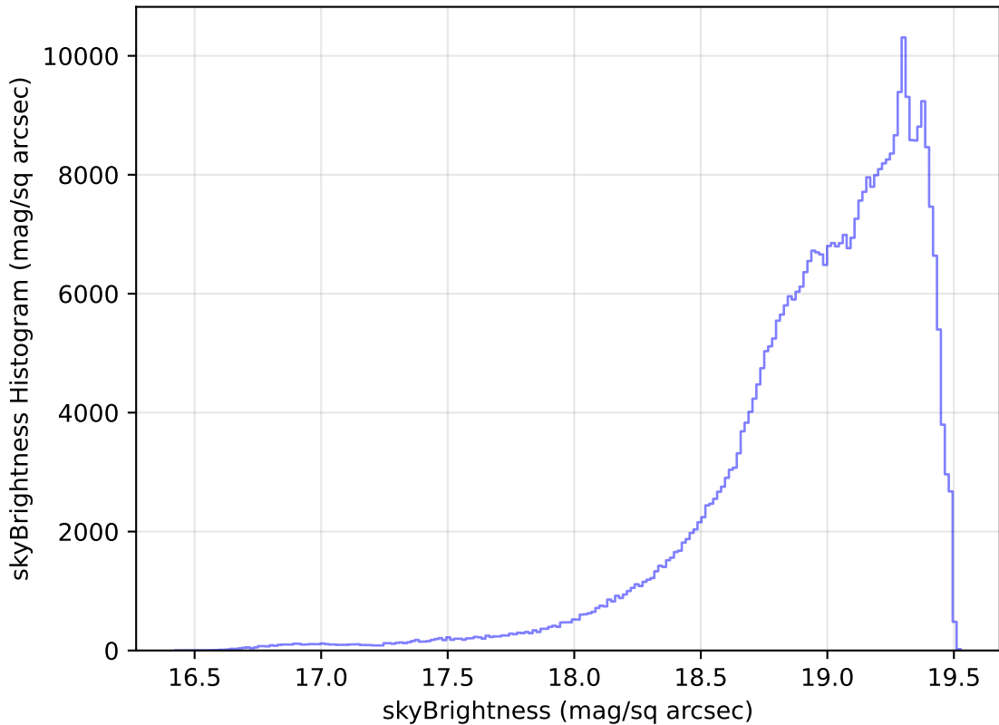
too_elab_r16_d2_ugrizy_v3.4_10yrs WFD z band: skyBrightness Histogram
