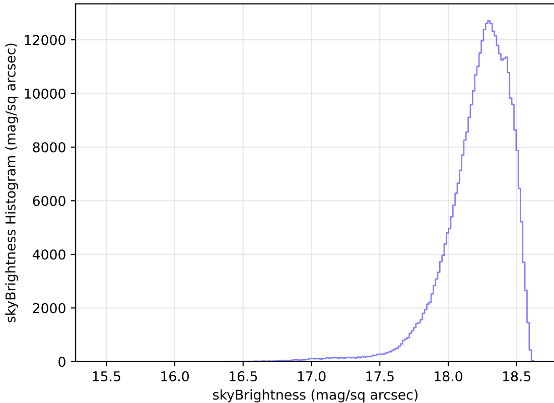
too_elab_r16_d2_ugrizy_v3.4_10yrs WFD y band: skyBrightness Histogram
