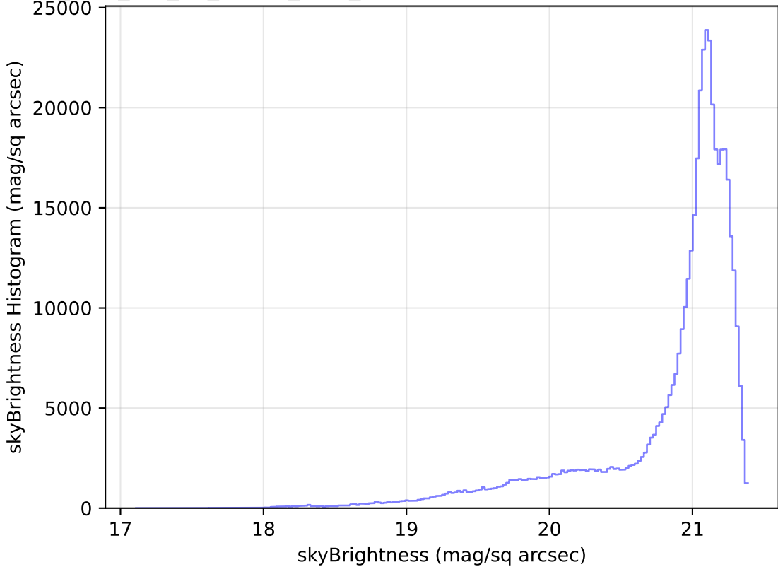
too_elab_r16_d2_ugrizy_v3.4_10yrs WFD r band: skyBrightness Histogram
