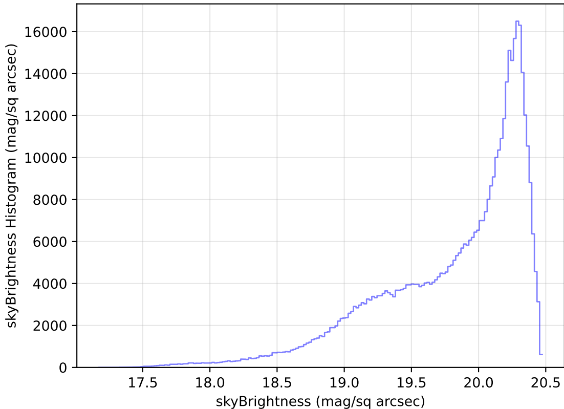
too_elab_r16_d2_ugrizy_v3.4_10yrs WFD i band: skyBrightness Histogram
