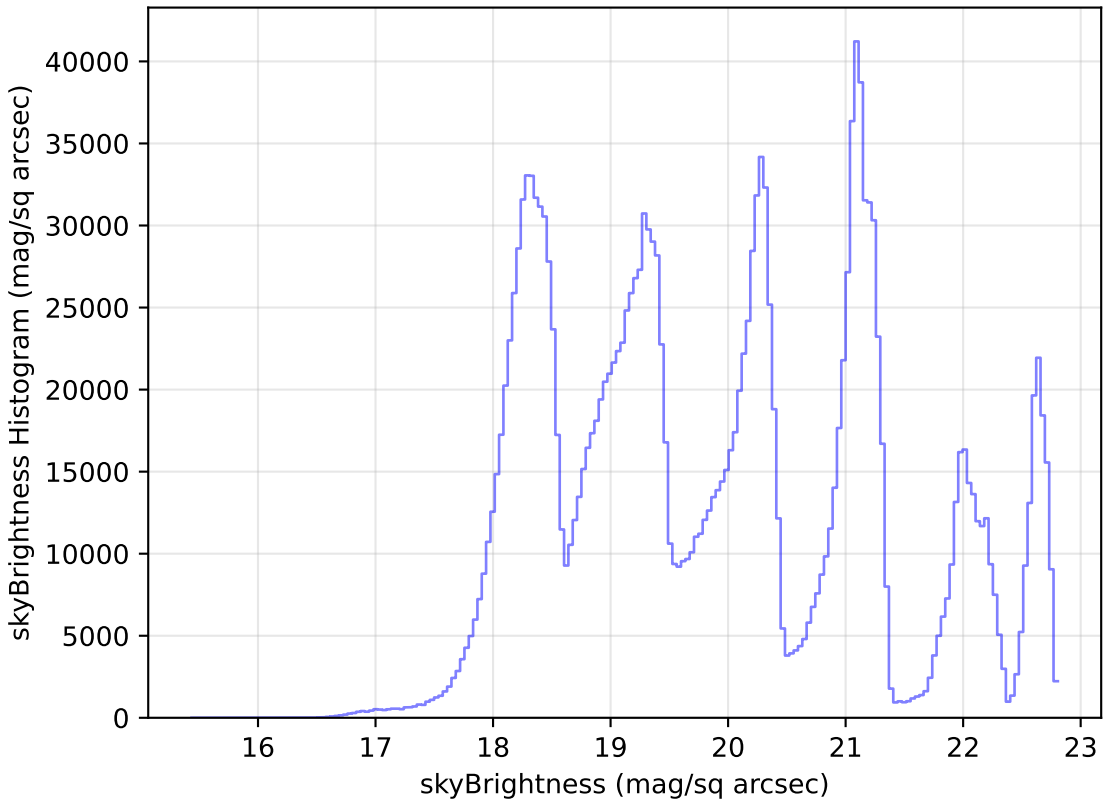
too_elab_r16_d2_ugrizy_v3.4_10yrs WFD all bands: skyBrightness Histogram
