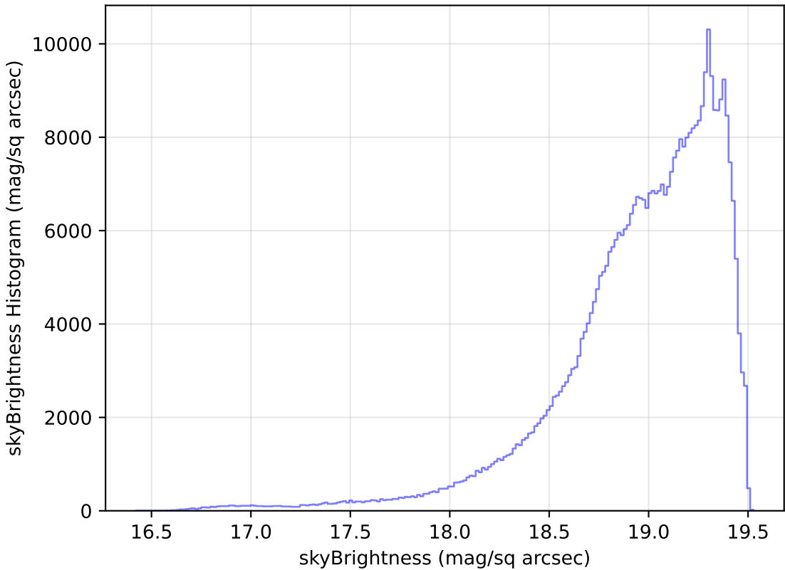
too_elab_r16_d2_ugrizy_v3.4_10yrs All sky z band: skyBrightness Histogram
