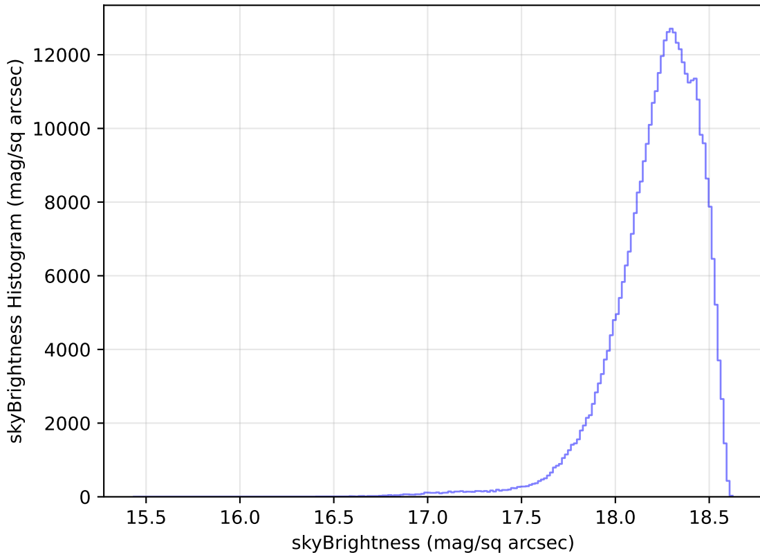
too_elab_r16_d2_ugrizy_v3.4_10yrs All sky y band: skyBrightness Histogram
