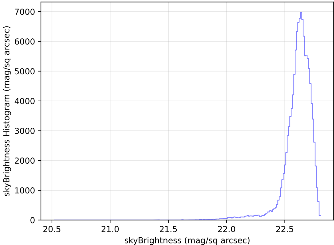
too_elab_r16_d2_ugrizy_v3.4_10yrs All sky u band: skyBrightness Histogram
