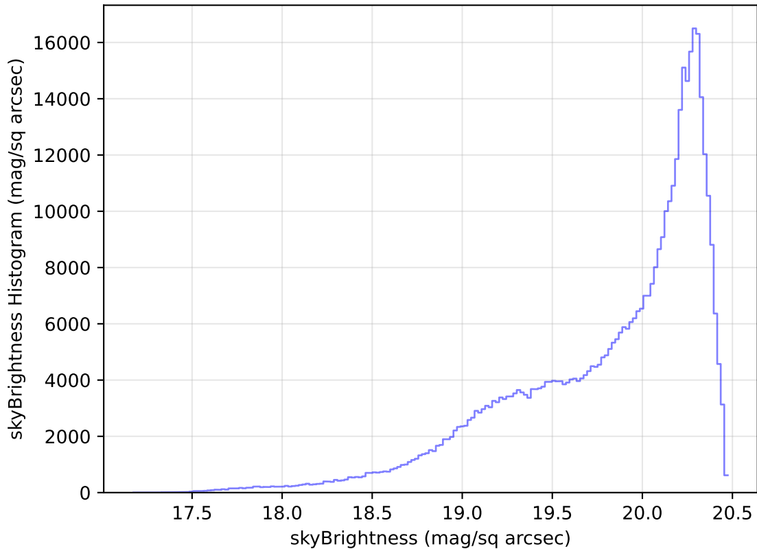
too_elab_r16_d2_ugrizy_v3.4_10yrs All sky i band: skyBrightness Histogram
