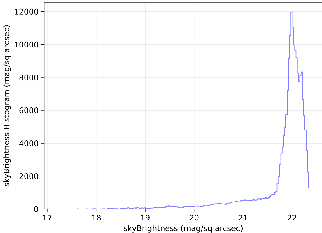
too_elab_r16_d2_ugrizy_v3.4_10yrs All sky g band: skyBrightness Histogram
