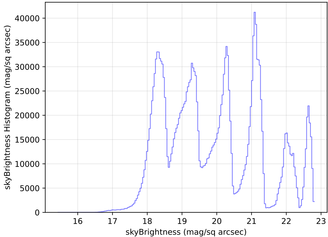
too_elab_r16_d2_ugrizy_v3.4_10yrs All sky all bands: skyBrightness Histogram
