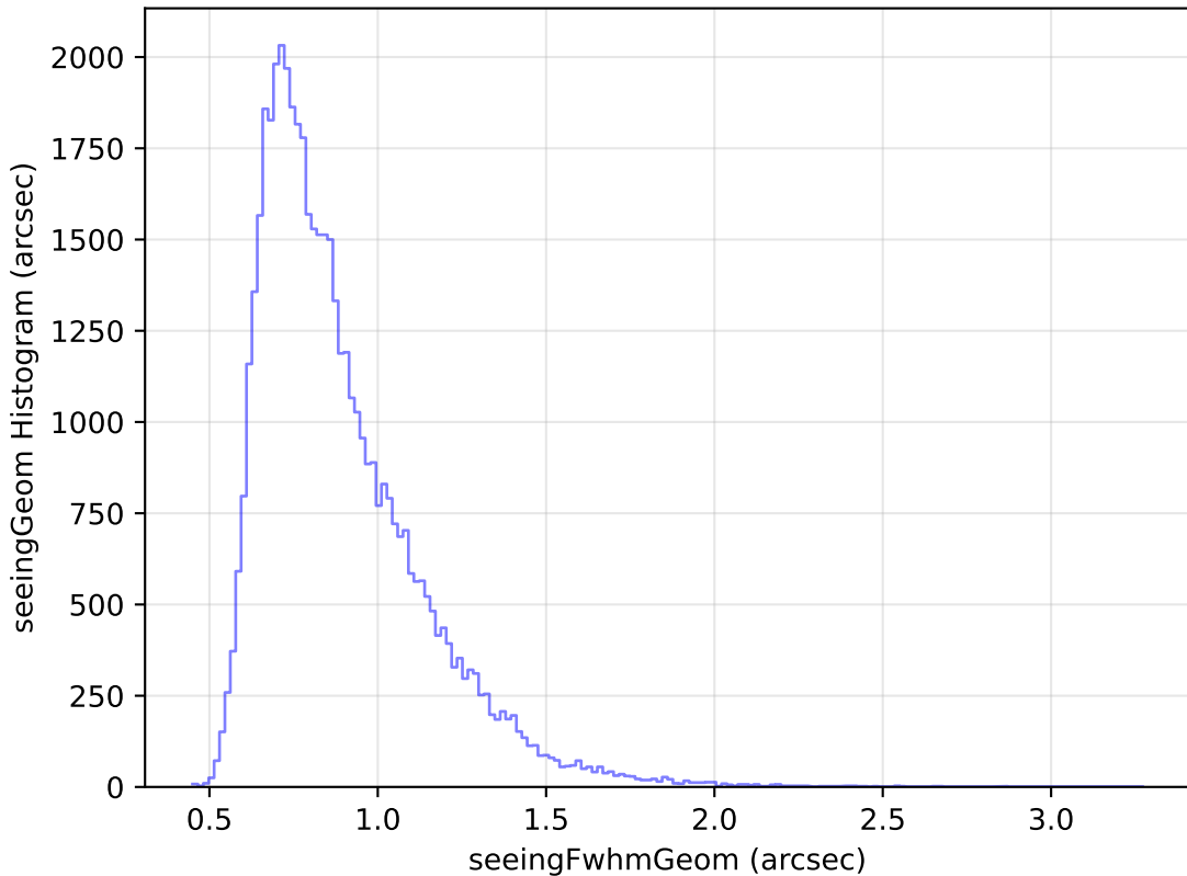
too_elab_r16_d2_ugrizy_v3.4_10yrs Yr 1 r band: seeingGeom Histogram
