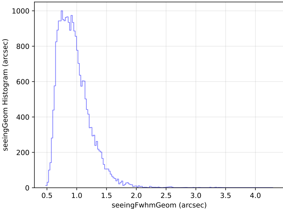
too_elab_r16_d2_ugrizy_v3.4_10yrs Yr 1 g band: seeingGeom Histogram
