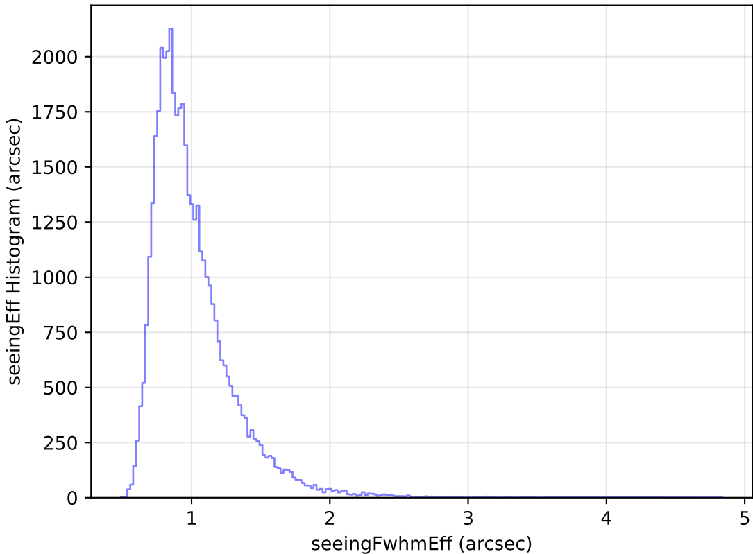
too_elab_r16_d2_ugrizy_v3.4_10yrs Yr 1 z band: seeingEff Histogram
