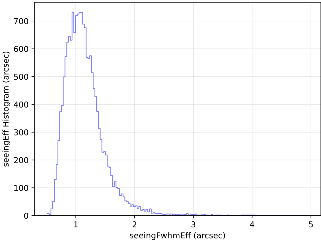
too_elab_r16_d2_ugrizy_v3.4_10yrs Yr 1 u band: seeingEff Histogram
