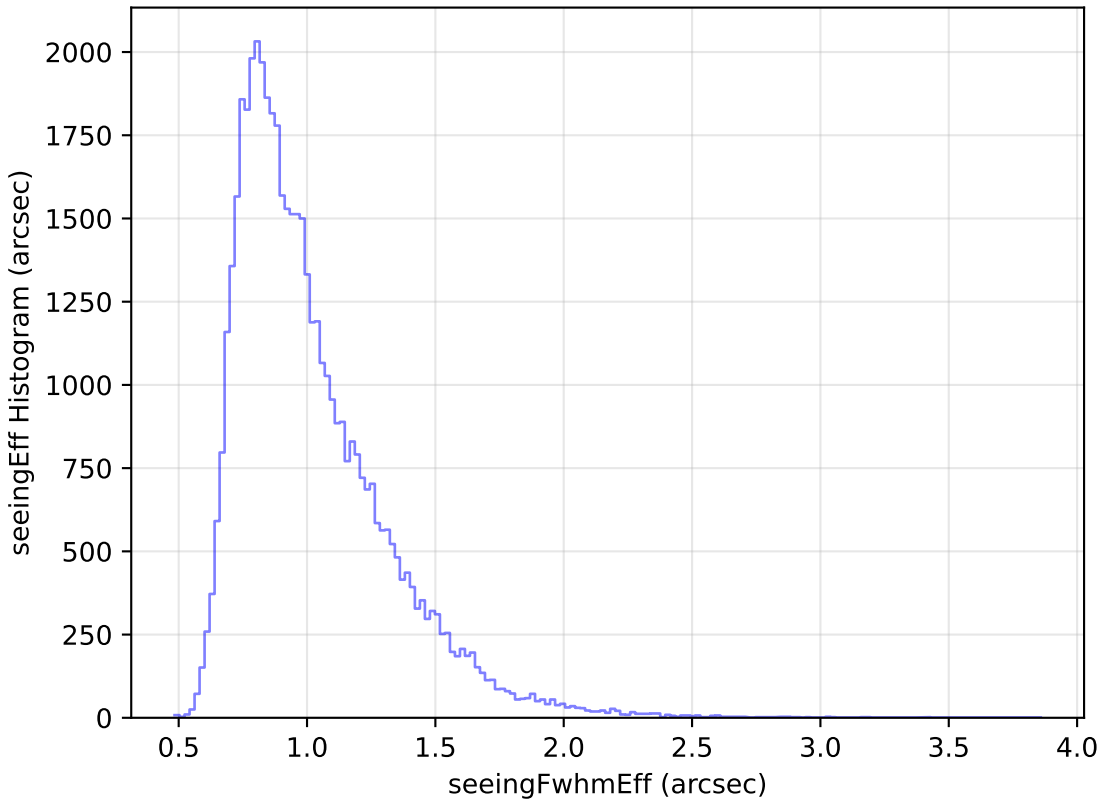
too_elab_r16_d2_ugrizy_v3.4_10yrs Yr 1 r band: seeingEff Histogram
