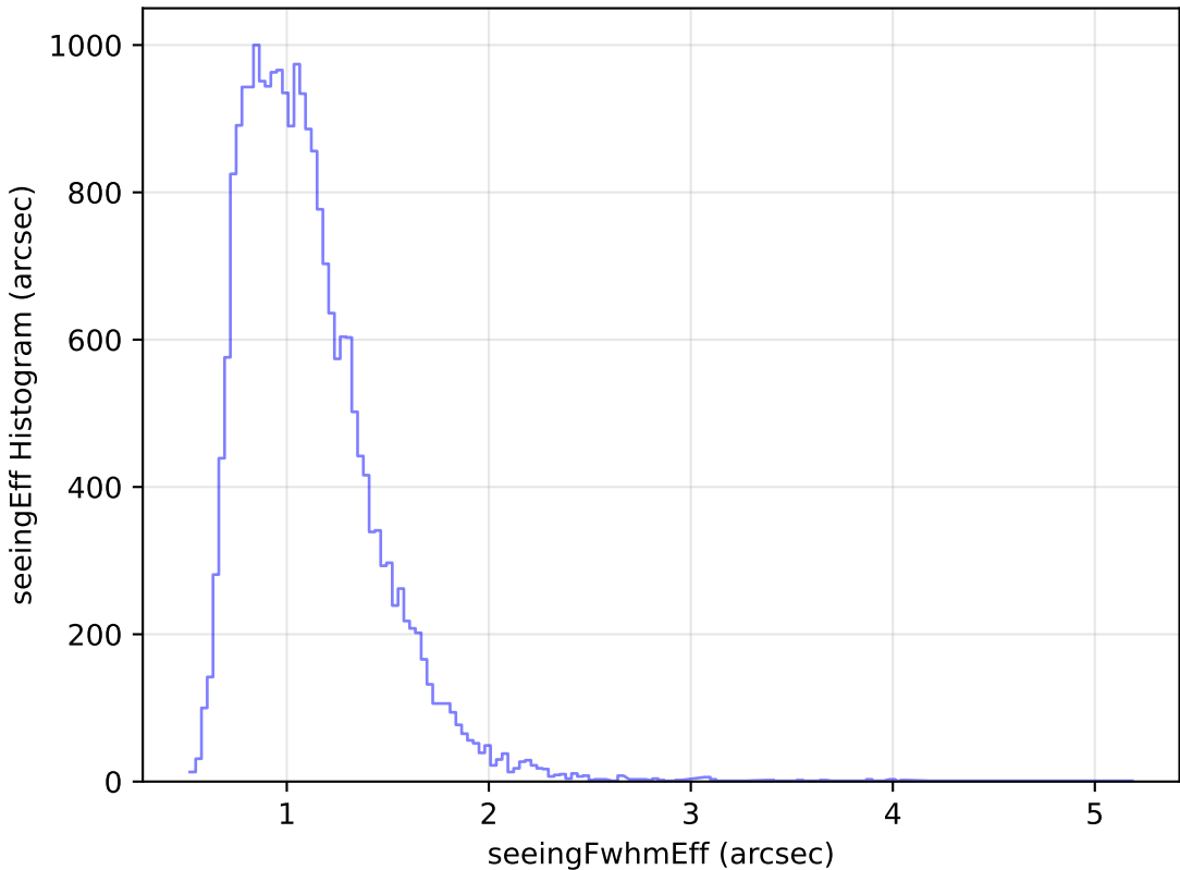
too_elab_r16_d2_ugrizy_v3.4_10yrs Yr 1 g band: seeingEff Histogram
