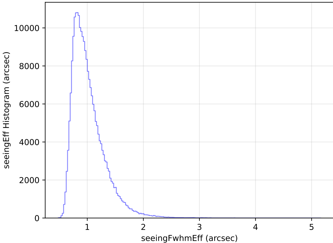
too_elab_r16_d2_ugrizy_v3.4_10yrs Yr 1 all bands: seeingEff Histogram
