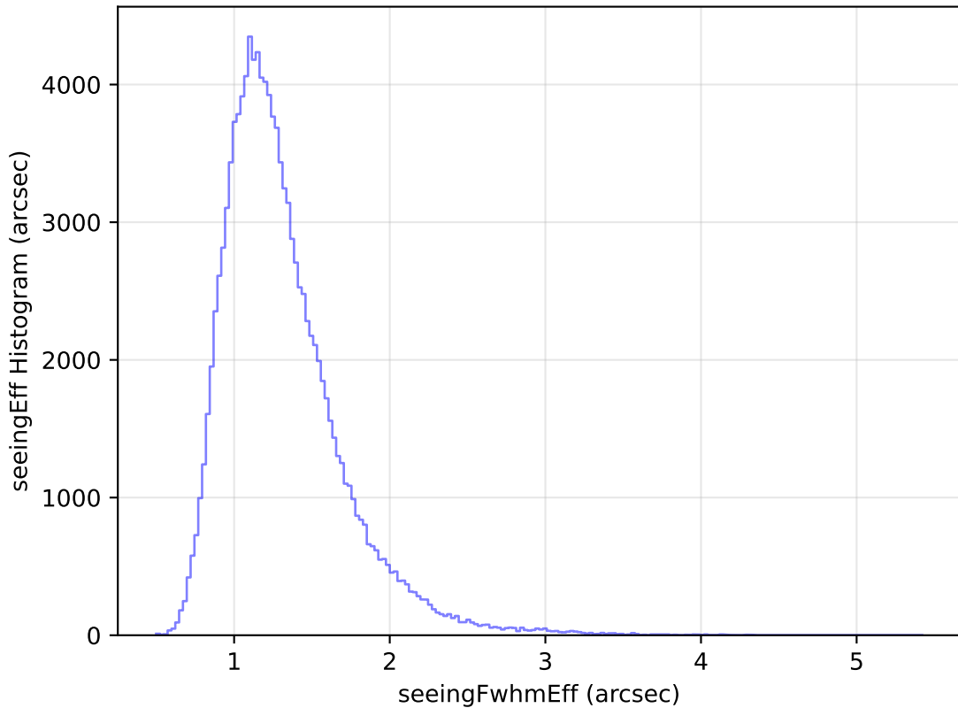
too_elab_r16_d2_ugrizy_v3.4_10yrs WFD u band: seeingEff Histogram
