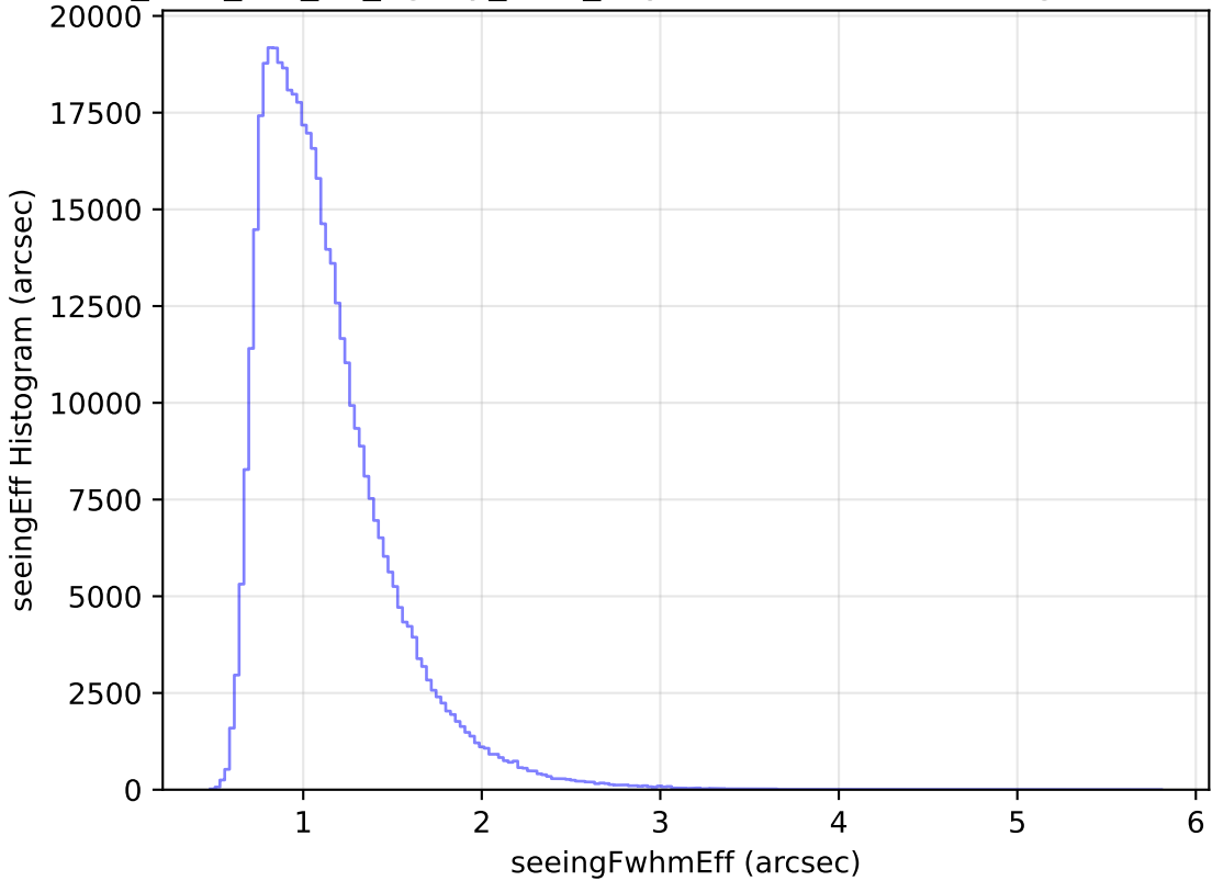
too_elab_r16_d2_ugrizy_v3.4_10yrs WFD r band: seeingEff Histogram
