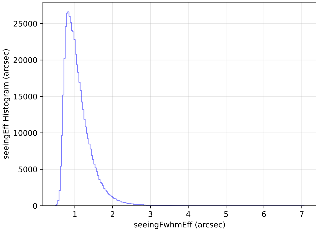
too_elab_r16_d2_ugrizy_v3.4_10yrs WFD i band: seeingEff Histogram
