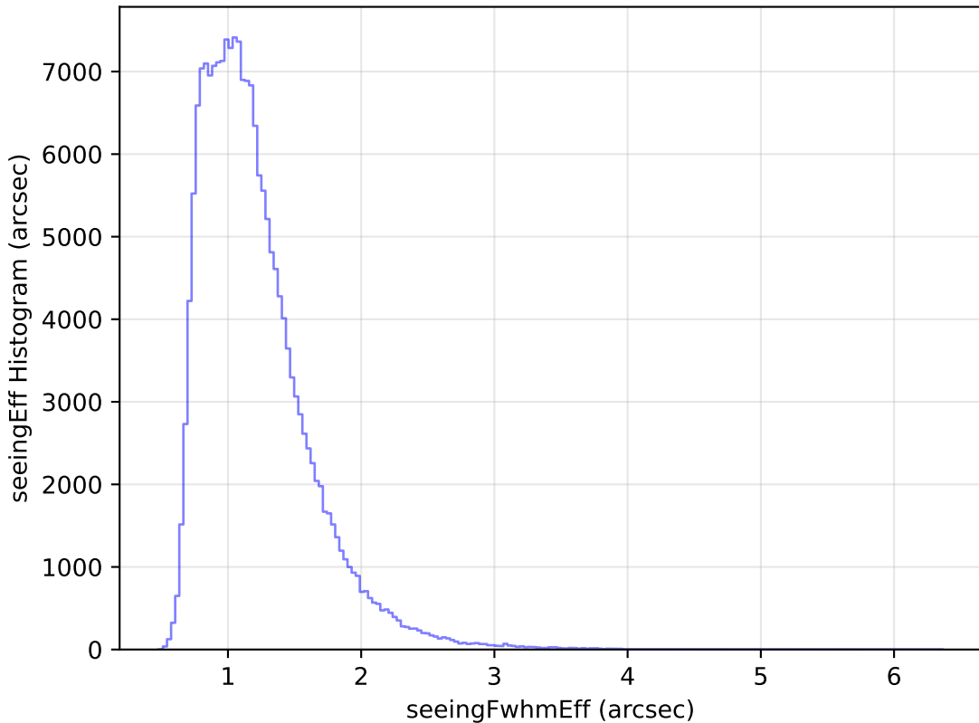
too_elab_r16_d2_ugrizy_v3.4_10yrs WFD g band: seeingEff Histogram
