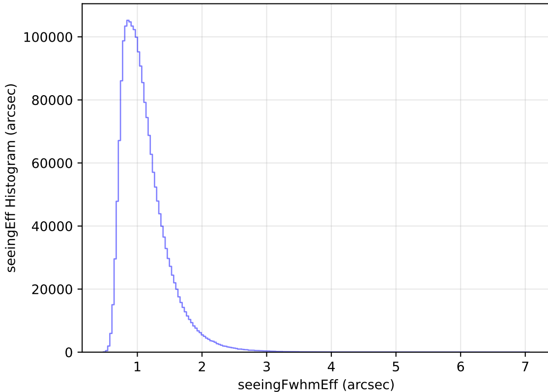
too_elab_r16_d2_ugrizy_v3.4_10yrs WFD all bands: seeingEff Histogram
