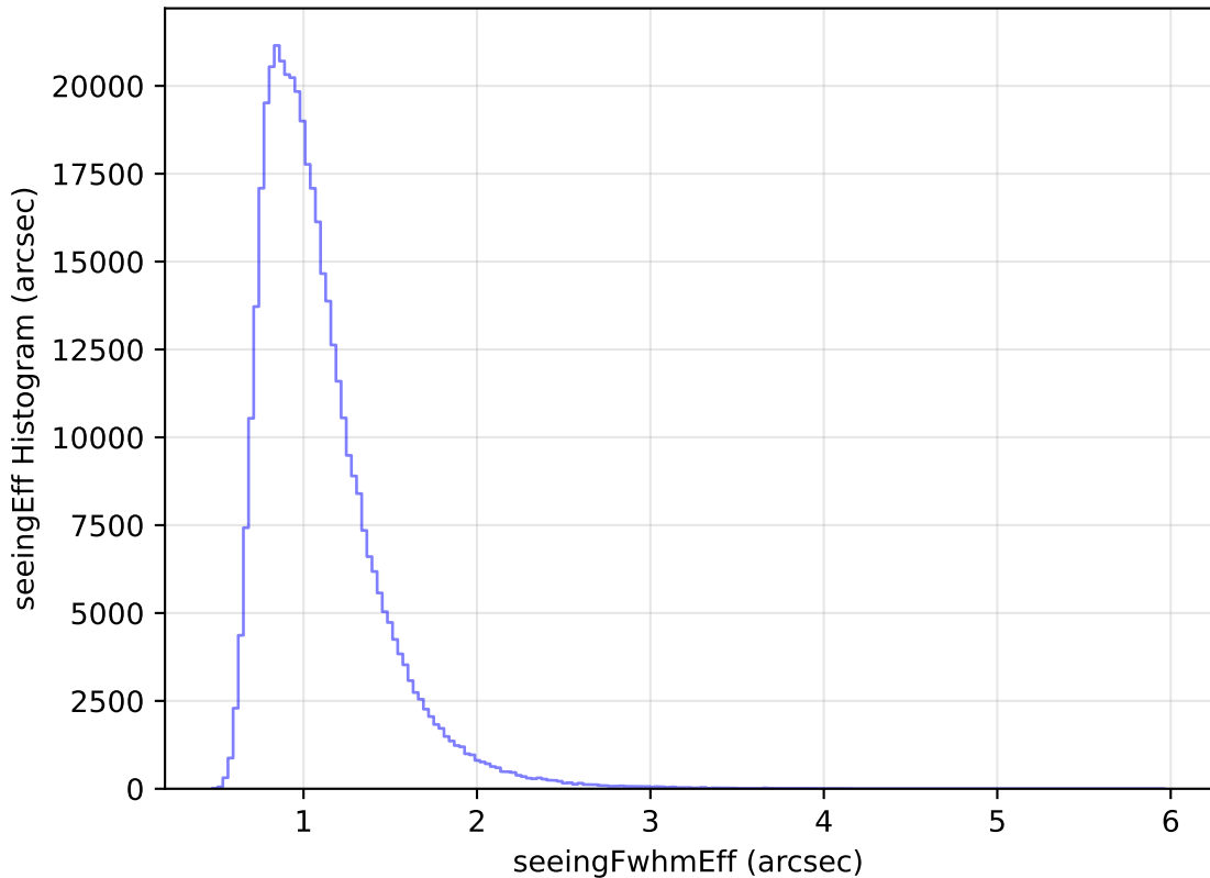
too_elab_r16_d2_ugrizy_v3.4_10yrs All sky z band: seeingEff Histogram
