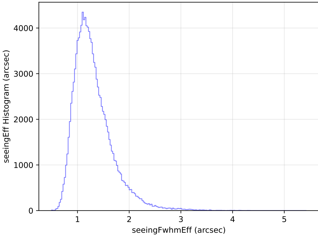
too_elab_r16_d2_ugrizy_v3.4_10yrs All sky u band: seeingEff Histogram
