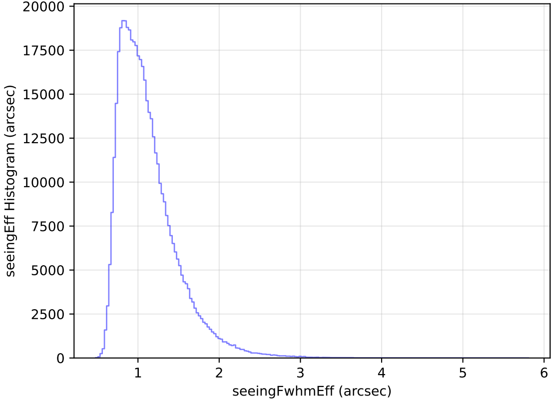
too_elab_r16_d2_ugrizy_v3.4_10yrs All sky r band: seeingEff Histogram
