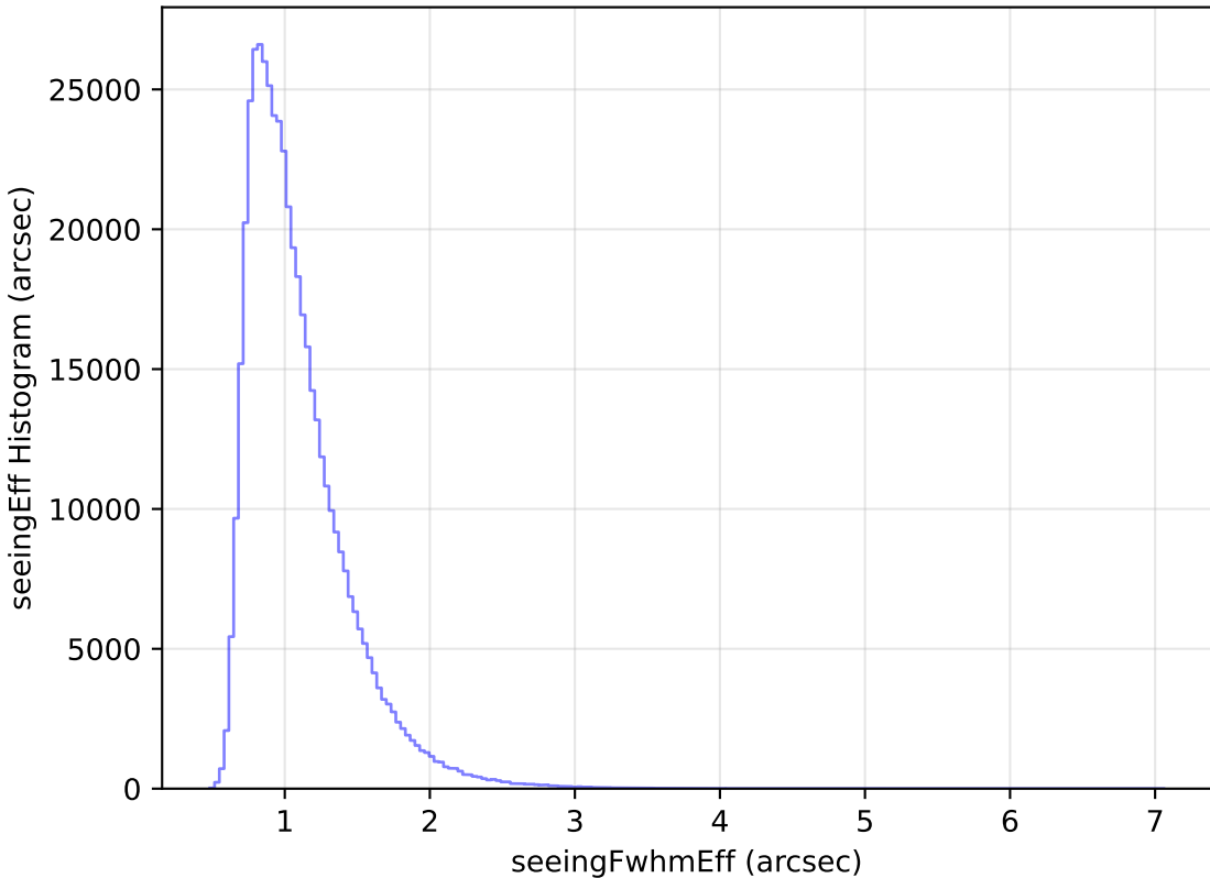
too_elab_r16_d2_ugrizy_v3.4_10yrs All sky i band: seeingEff Histogram
