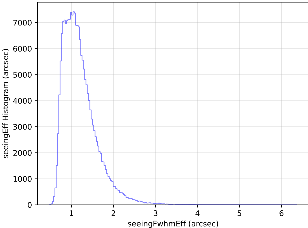
too_elab_r16_d2_ugrizy_v3.4_10yrs All sky g band: seeingEff Histogram
