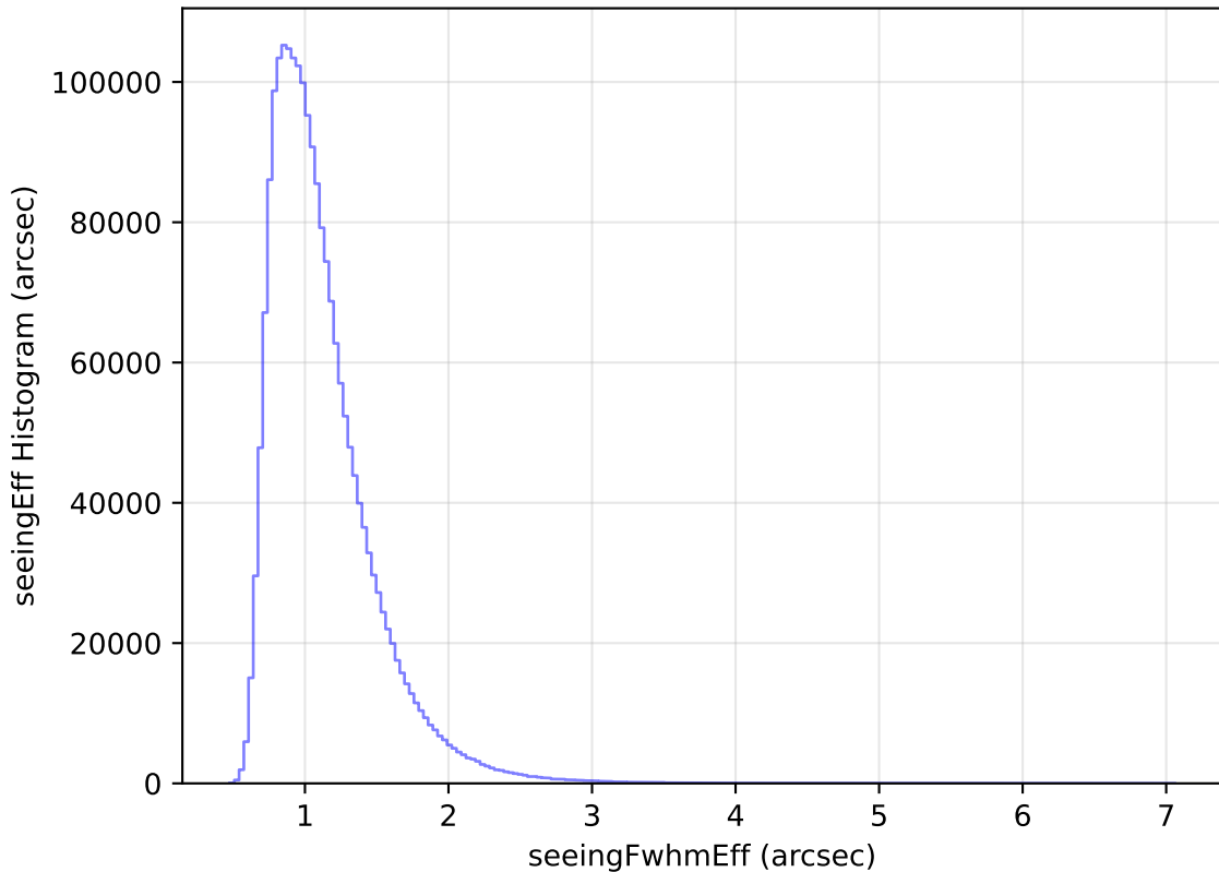
too_elab_r16_d2_ugrizy_v3.4_10yrs All sky all bands: seeingEff Histogram
