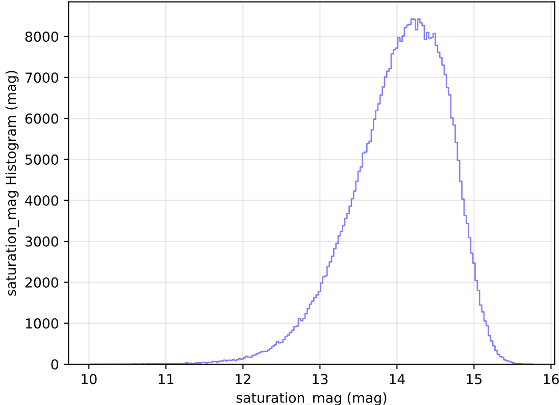
too_elab_r16_d2_ugrizy_v3.4_10yrs WFD z band: saturation_mag Histogram
