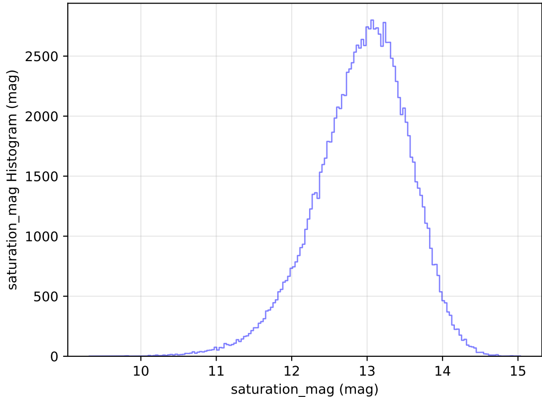
too_elab_r16_d2_ugrizy_v3.4_10yrs WFD u band: saturation_mag Histogram
