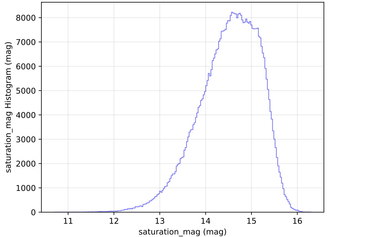
too_elab_r16_d2_ugrizy_v3.4_10yrs WFD r band: saturation_mag Histogram
