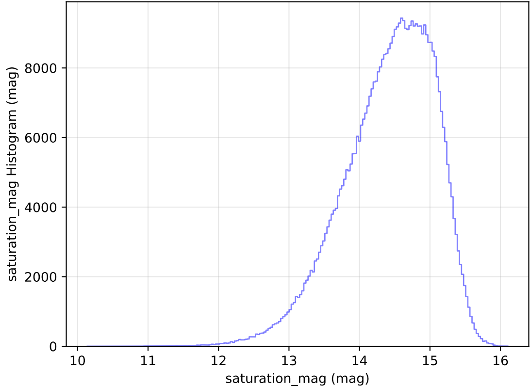
too_elab_r16_d2_ugrizy_v3.4_10yrs WFD i band: saturation_mag Histogram
