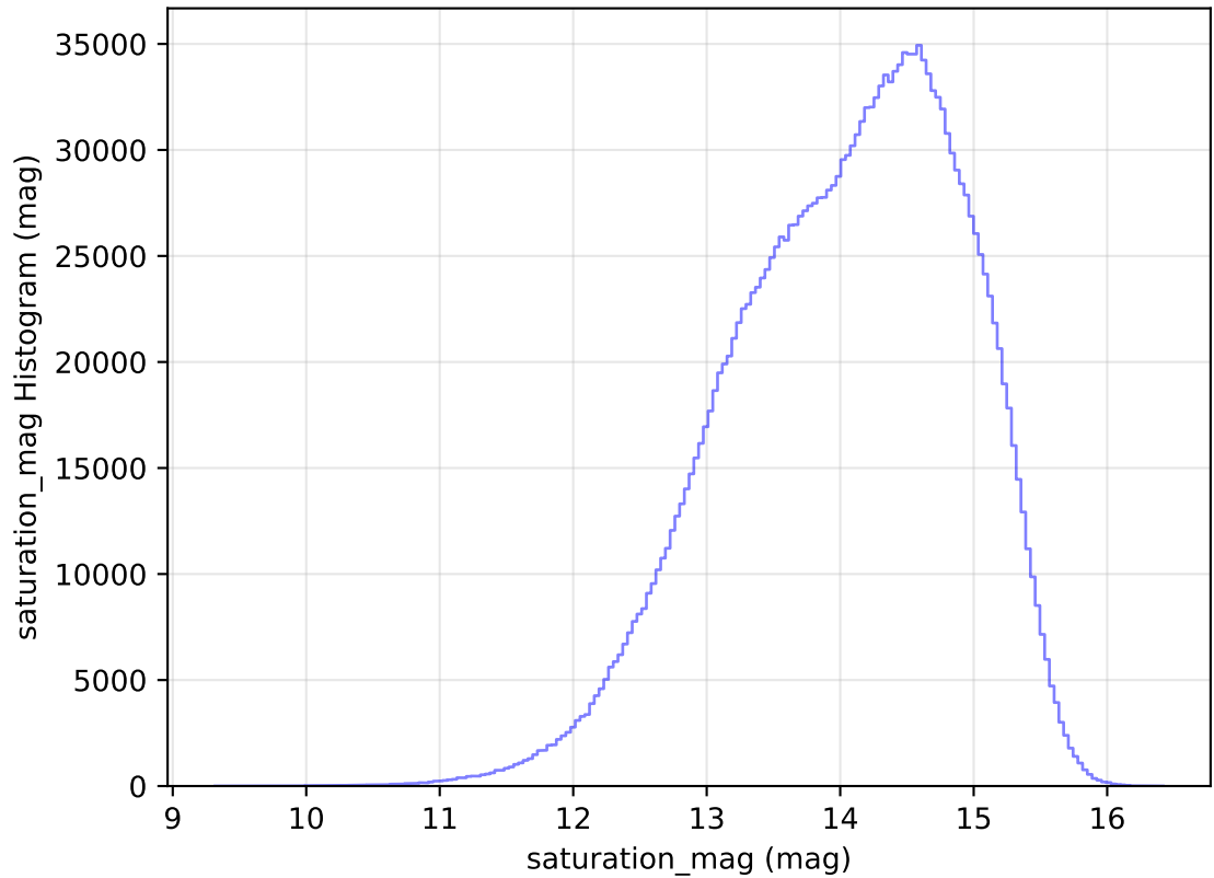
too_elab_r16_d2_ugrizy_v3.4_10yrs WFD all bands: saturation_mag Histogram
