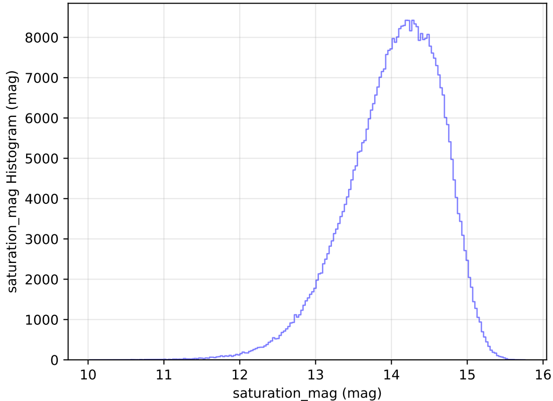
too_elab_r16_d2_ugrizy_v3.4_10yrs All sky z band: saturation_mag Histogram
